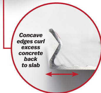
Cutting Rear Profile
