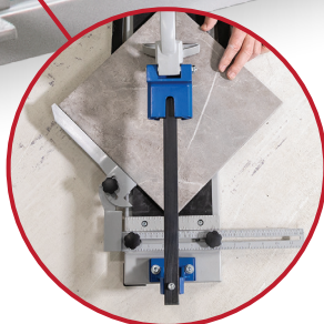
Protractor Gauge for Angled Cuts
